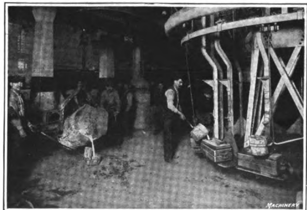
Fig. 32—To facilitate pouring metal into molds in the Ford Motor Co.'s foundry, molds are brought in on a conveyor and transferred to a carousel on which each mold is supported by a pendulum. This swinging support eliminates vibration and prevents molds breaking. Molds are carried away by a second conveyor
